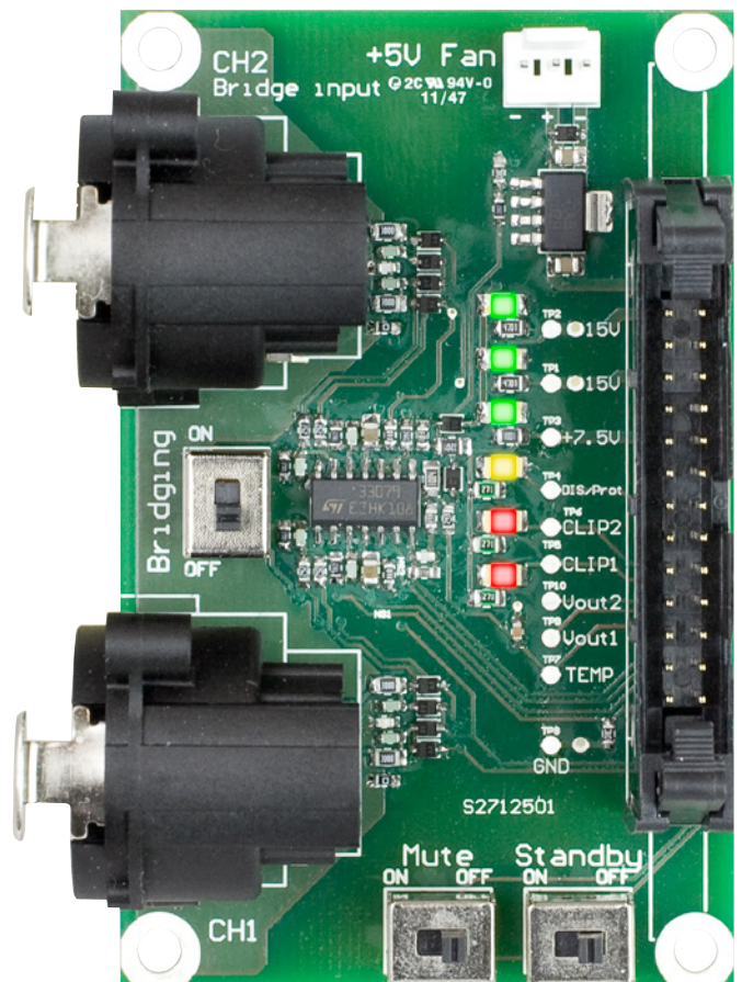
The enclosed I/O-board provide easy connection of input signals, LED status indicators, control switches for relevant functions as well as PCB measurements points.
