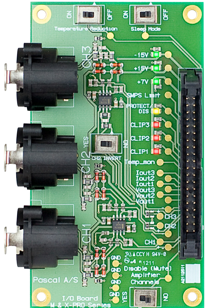
The enclosed I/O-board provide easy connection of input signals, LED status indicators, control switches for relevant functions as well as PCB measurements points.
