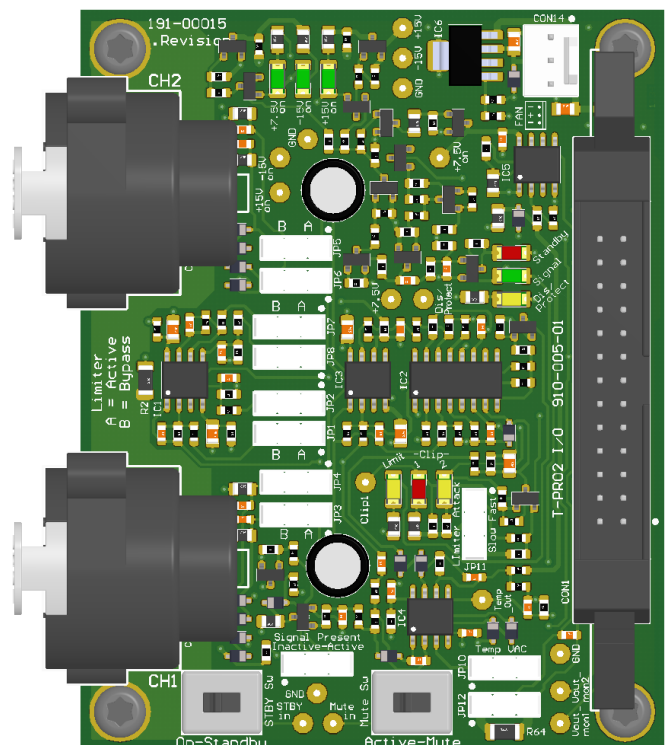
The enclosed I/O-board provide easy connection of input signals, LED status indicators, control switches for relevant functions as well as PCB measurements points.
